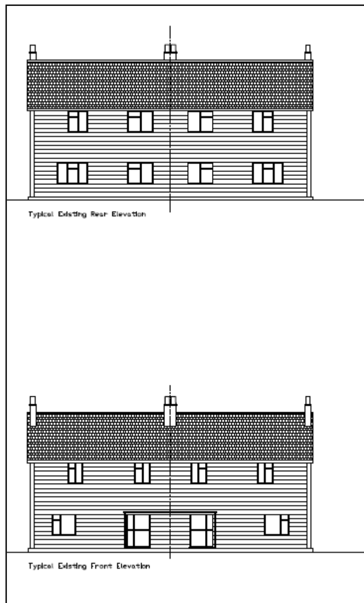
Figure 3 existing front and rear elevations
